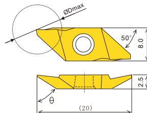
TBP ØDmax=Ø5~10mm
